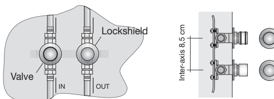
Connection of Remote Valve Assembly (GVR) to water system
